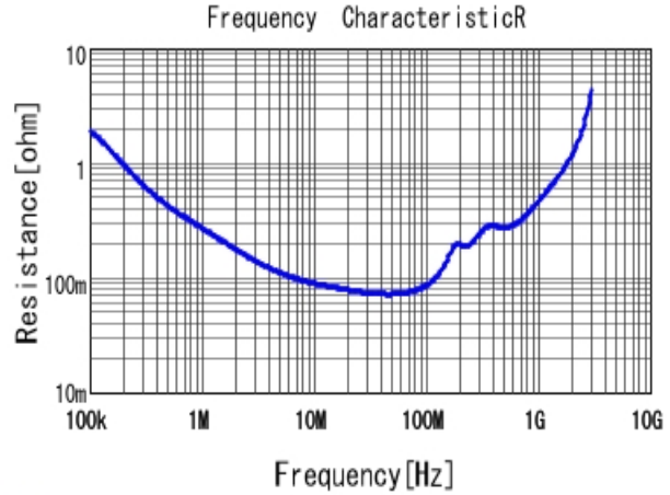
■ GRJ32QR73A103KWJ1 R DCOV, 25degC
