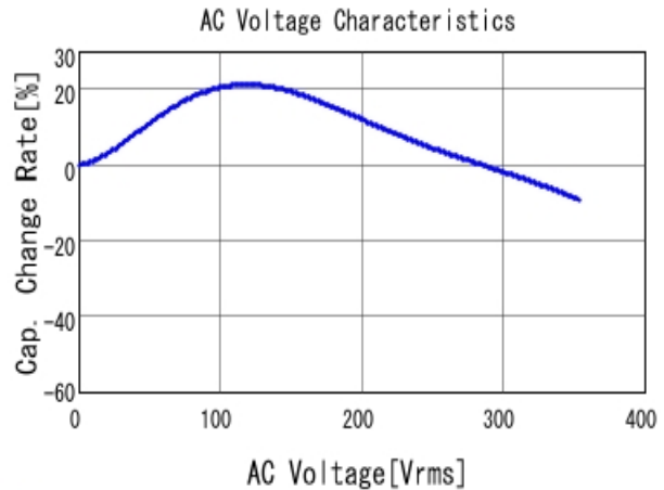
■ GRJ32QR73A103KWJ1 C-AC Voltage capchange, DCOV, 25.0d
