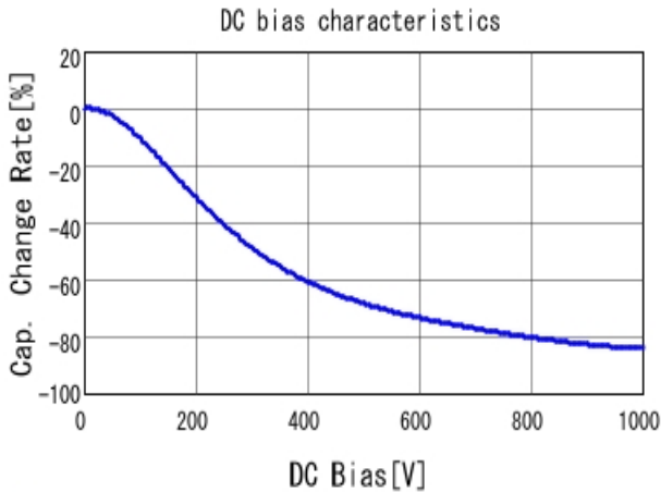
■ GRJ32QR73A103KWJ1 C-DC bias capchange, 25.0degC, AC1V
