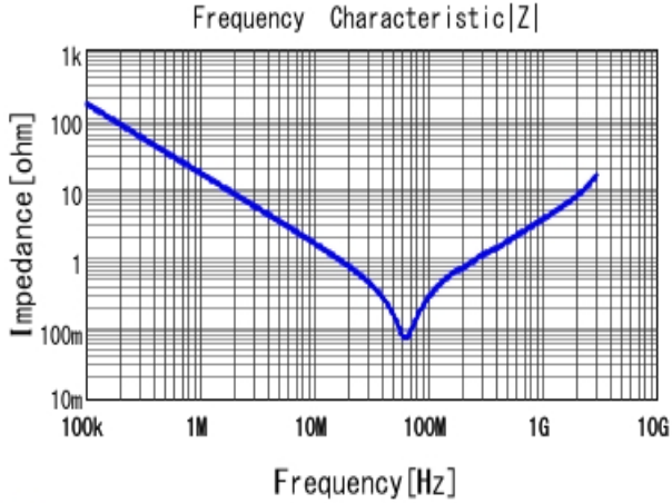
■ GRJ32QR73A103KWJ1 |Z| DCOV, 25degC
