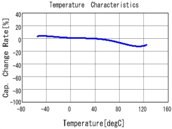
■ GRJ32QR73A103KWJ1 C-Temp. capchange, DCOV, AC1Vrms
