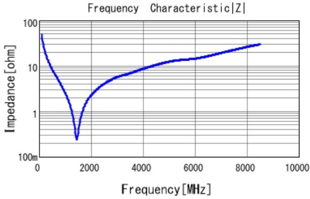
GRM1555C1H330GA01 |Z| DCOV, 25degC
