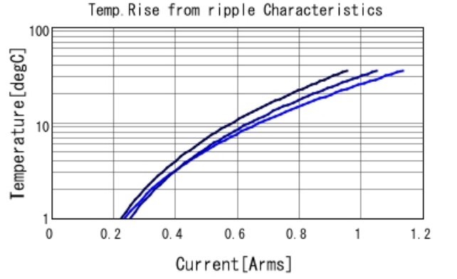
GRM1555C1H330GA01 Temp. rise — 500MHz — 700I
