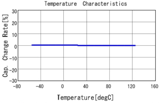
GRM1555C1H330GA01 C-Temp. capchange, DCOV, AC1Vrms
