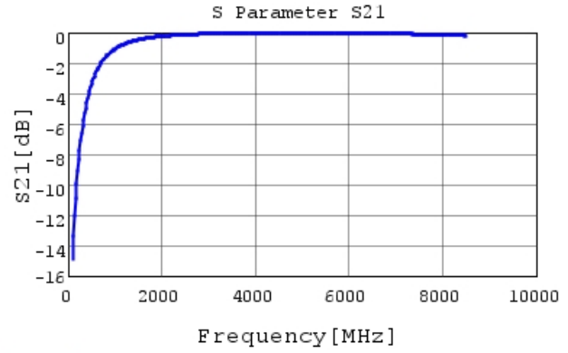
GCQ1555C1H2R9CB01 S21 DCOV, 25degC
