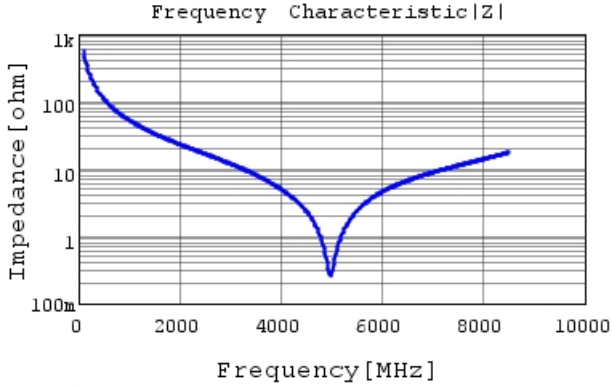
GCQ1555C1H2R9CB01 |Z| DC0V, 25degC
