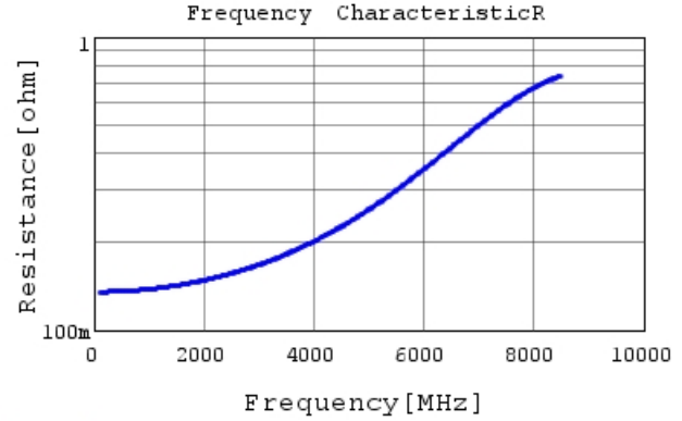
GCQ1555C1H2R9CB01 R DC0V, 25degC
