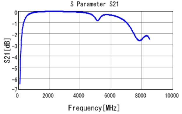
GRM1885C2A8R5BA01 S21 DCOV, 25degC
