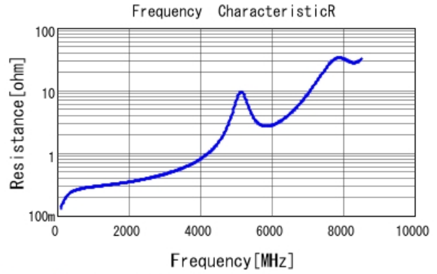
GRM1885C2A8R5BA01 R DCOV, 25degC
