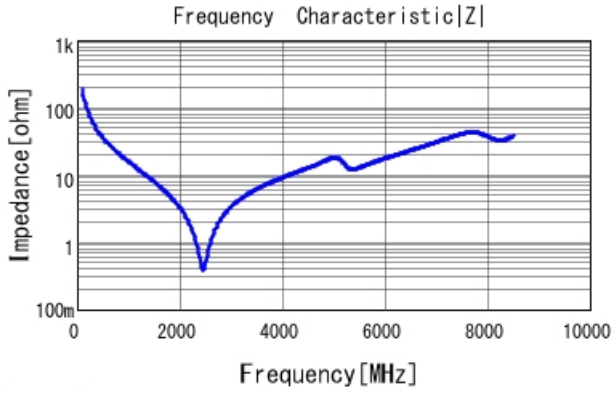
GRM1885C2A8R5BA01 |Z| DCOV, 25degC
