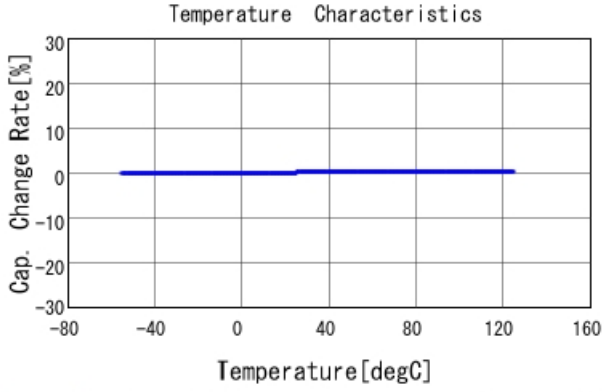
GRM1885C2A8R5BA01 C-Temp. capchange, DCOV, AC1Vrms
