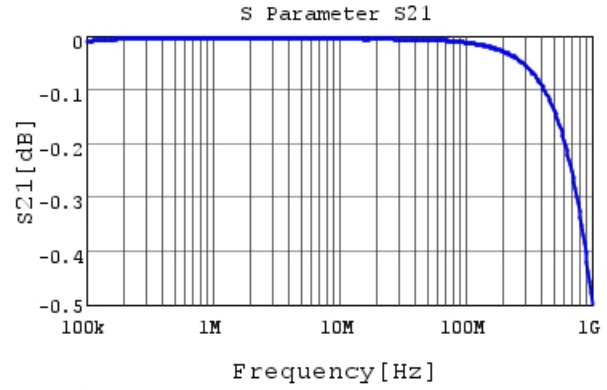
RCER72A474K2K1H03B S21 DC0V, 25degC
