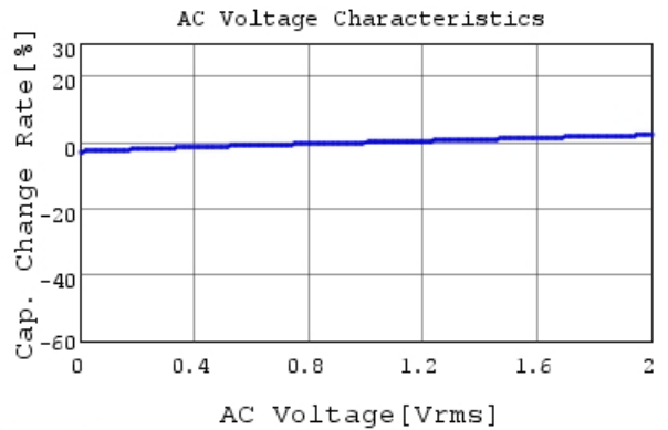
RCER72A474K2K1H03B C-AC Voltage capchange, I
