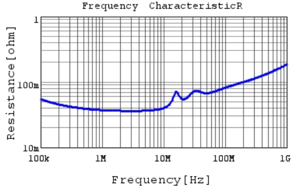
RCER72A474K2K1H03B R DC0V, 25degC
