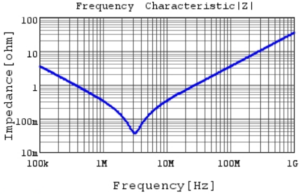
RCER72A474K2K1H03B |Z| DC0V, 25degC
