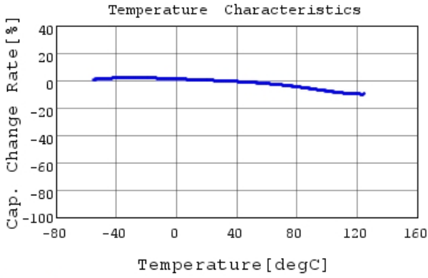
RCER72A474K2K1H03B C-Temp. capchange, DC0.0V
