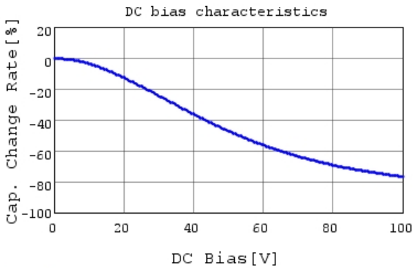
RCER72A474K2K1H03B C-DC bias capchange, 25.0
