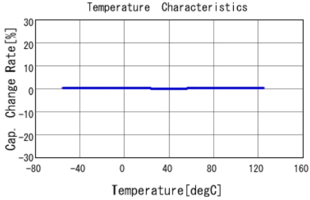
GRM1555C2A4R6WA01 C-Temp. capchange, DCOV, AC1Vrms
