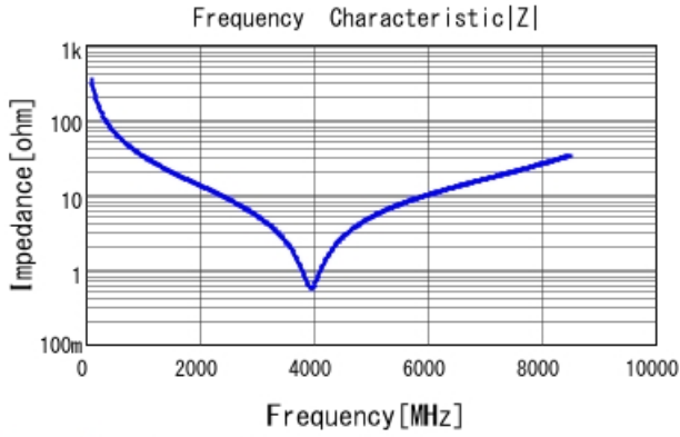
GRM1555C2A4R6WA01 |Z| DCOV, 25degC
