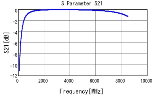
GRM1555C2A4R6WA01 S21 DCOV, 25degC
