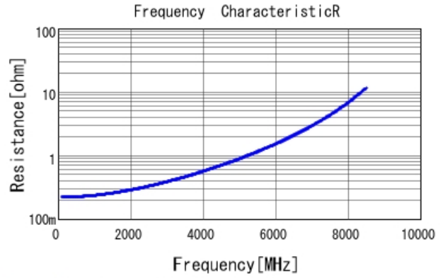
GRM1555C2A4R6WA01 R DCOV, 25degC
