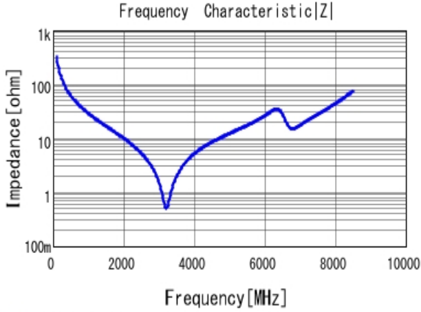
■ GRM1885C1H5R0CA01 |Z| DCOV, 25degC
