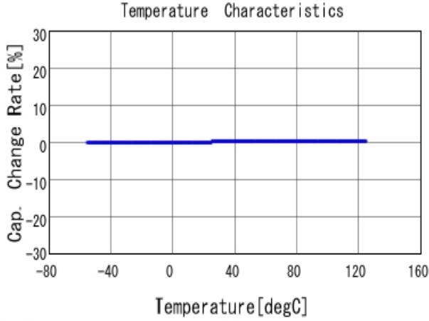
■ GRM1885C1H5R0CA01 C-Temp. capchange, DCOV, AC1Vrms
