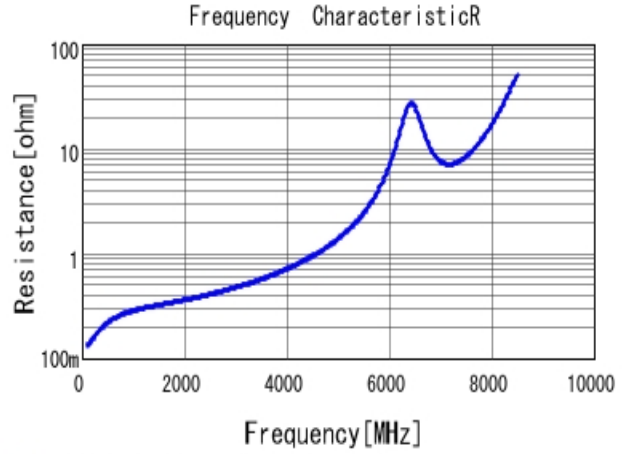
■ GRM1885C1H5R0CA01 R DCOV, 25degC
