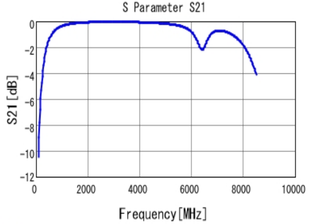
■ GRM1885C1H5R0CA01 S21 DCOV, 25degC
