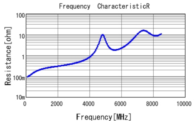
GRM1885C2A9R7DA01 R DCOV, 25degC
