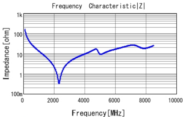
GRM1885C2A9R7DA01 |Z| DCOV, 25degC
