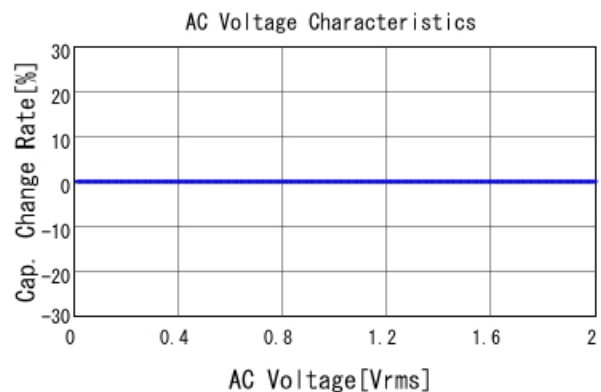
GRM1885C2A9R7DA01 C-AC Voltage capchange, DCOV, 25
