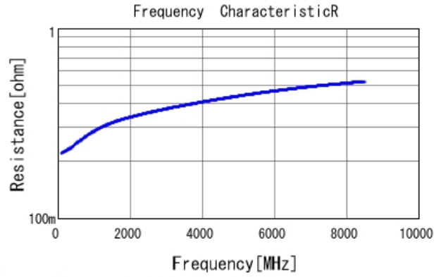
GRM0225C1E2R3BA03 R DCOV, 25degC
