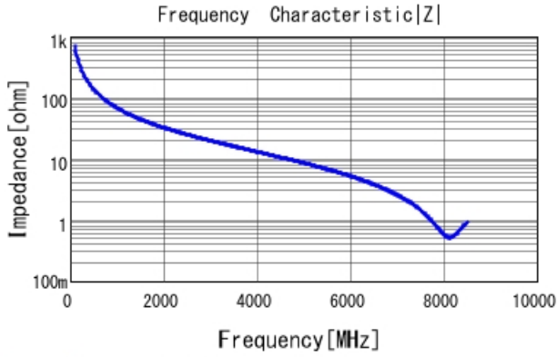
GRM0225C1E2R3BA03 |Z| DCOV, 25degC
