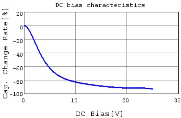
GRM033R61E224KE01 C-DC bias capchange, 25.0c
