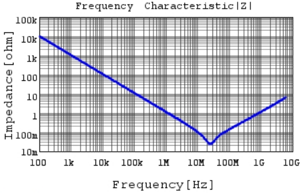
GRM033R61E224KE01 |Z| DCOV, 25degC
