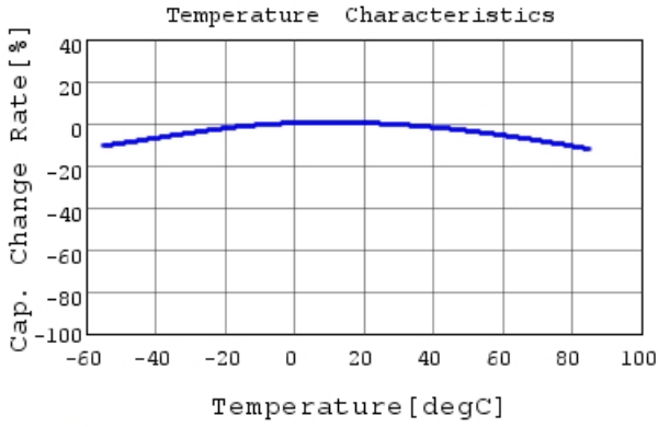
GRM033R61E224KE01 C-Temp. capchange, DC0.0V,
