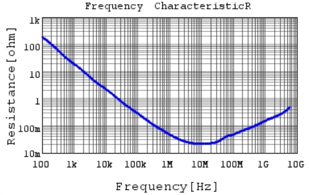
GRM033R61E224KE01 R DCOV, 25degC
