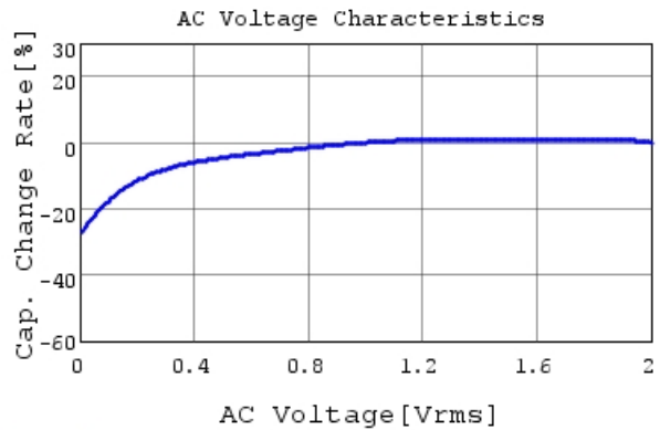
GRM033R61E224KE01 C-AC Voltage capchange, Dc
