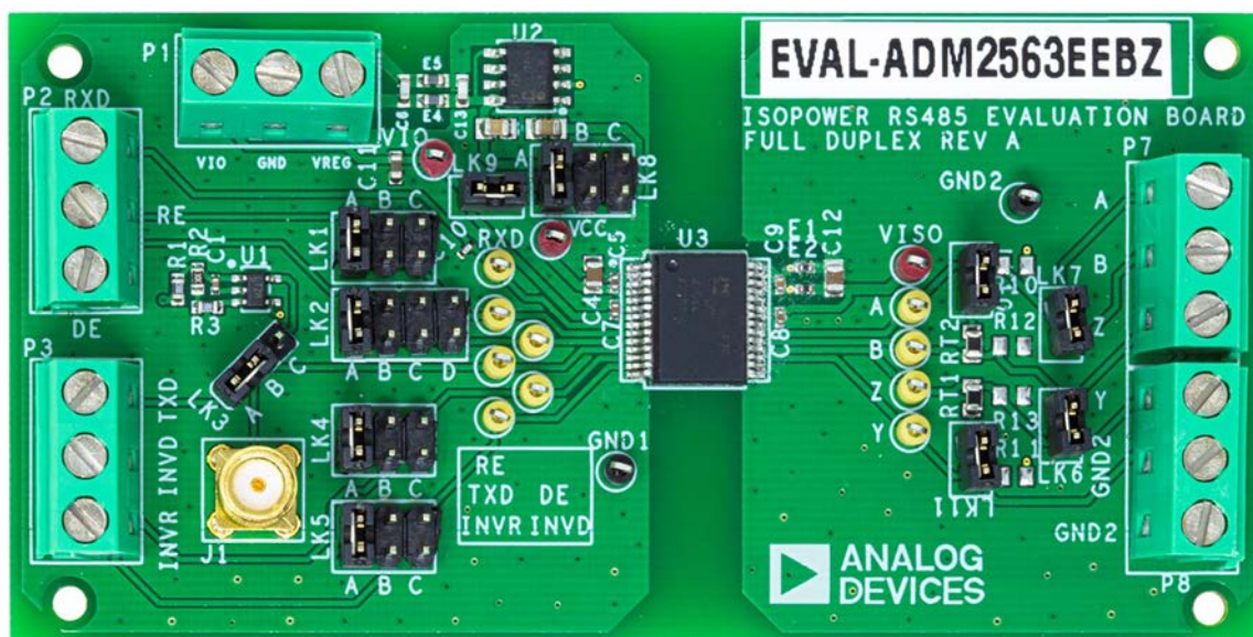
Figure 1. EVAL-ADM2563EEBZ
