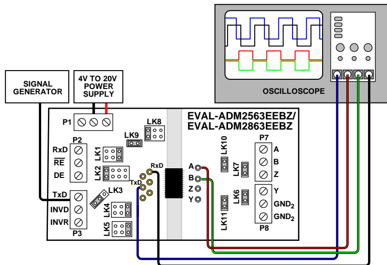
Figure 5. Full-Duplex RS-485 Transceiver Loopback Test
