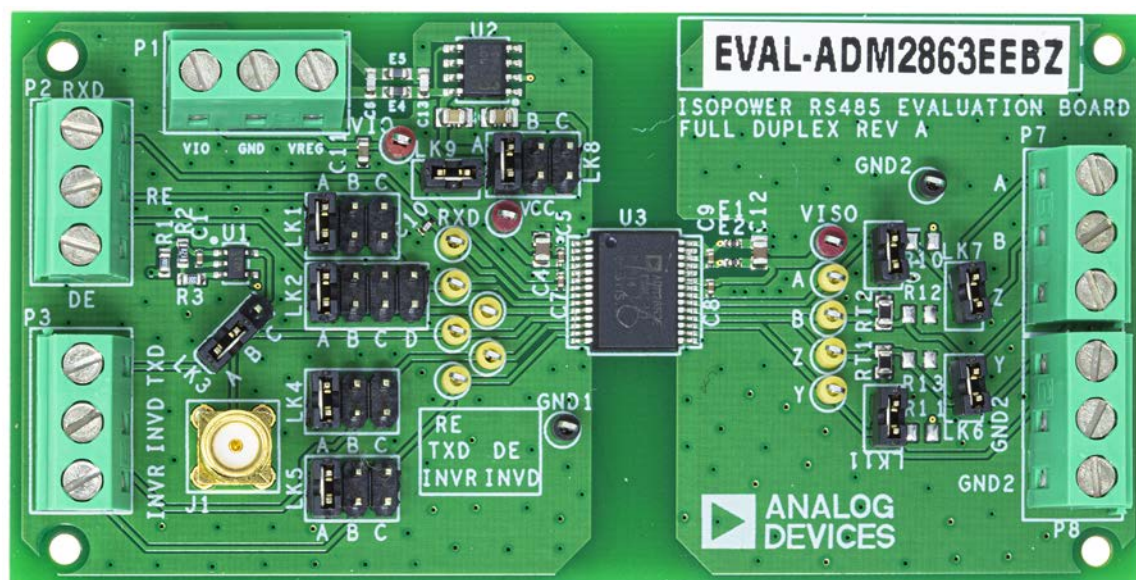
Figure 2. EVAL-ADM2863EEBZ
