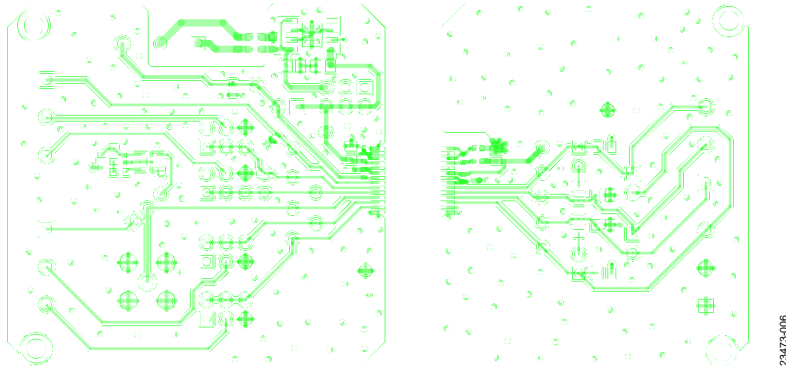
Figure 9. EVAL-ADM2563EEBZ/EVAL-ADM2863EEBZ Component Side, Layer 1
