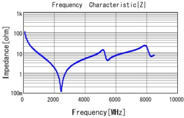
GQM1555C2D150JB01 |Z| DCOV, 25degC
