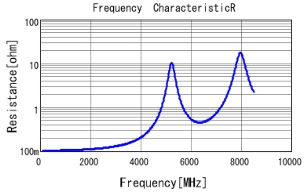
GQM1555C2D150JB01 R DCOV, 25degC
