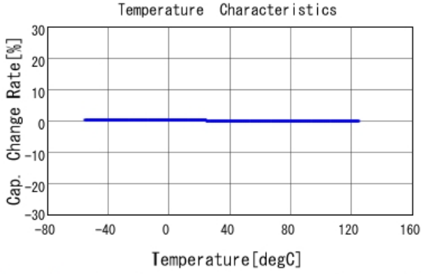
GQM1555C2D150JB01 C-Temp. capchange, DCOV, AC1Vrms
