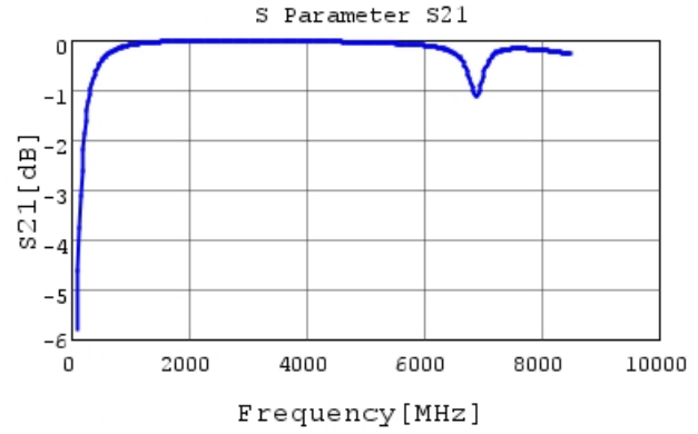
GCQ1555C1H9R5WB01 S21 DCOV, 25degC
