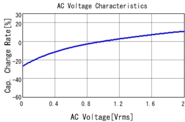
GRM219R61H105KA73 C-AC Voltage capchange, DCOV, 25
