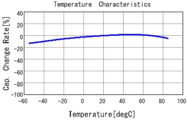
GRM219R61H105KA73 C-Temp. capchange, DC0.0V, AC1.C
