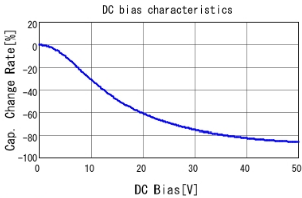
GRM219R61H105KA73 C-DC bias capchange, 25.0degC, A
