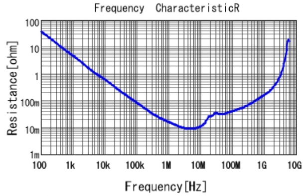
GRM219R61H105KA73 R DCOV, 25degC
