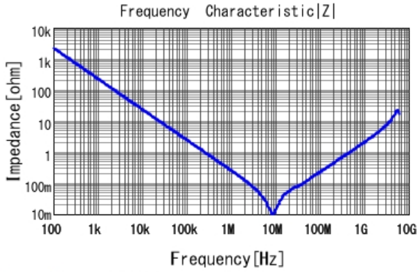
GRM219R61H105KA73 |Z| DCOV, 25degC
