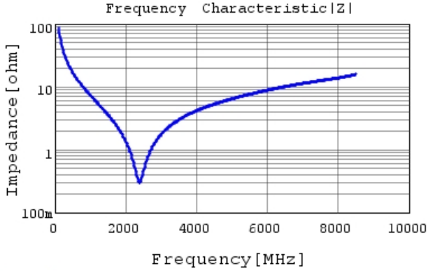
GRM0335C1H180JA01 |Z| DCOV, 25degC
