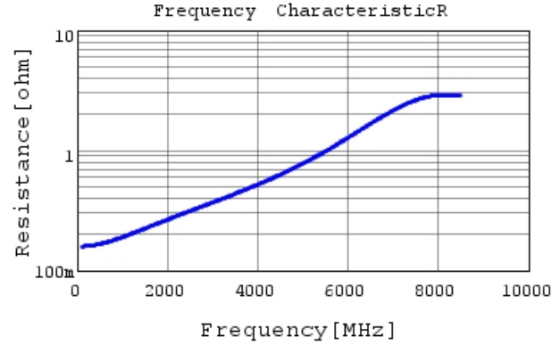
GRM0335C1H180JA01 R DCOV, 25degC
