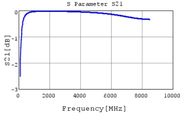
GRM0335C1H180JA01 S21 DCOV, 25degC
