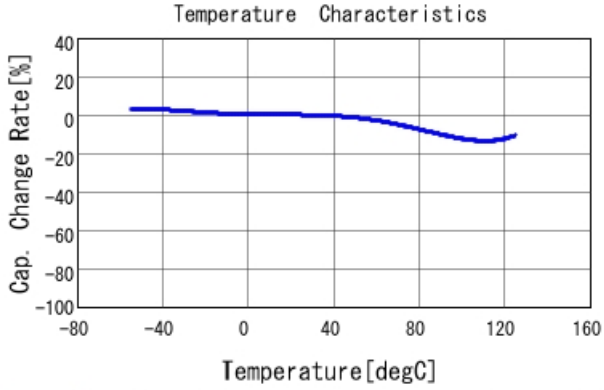
GRM31AR72J222KW01 C-Temp. capchange, DCOV, AC1Vrms
