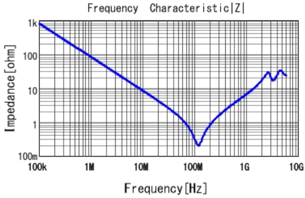
GRM31AR72J222KW01 |Z| DCOV, 25degC
