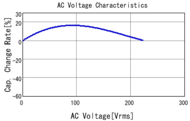
GRM31AR72J222KW01 C-AC Voltage capchange, DCOV, 25
