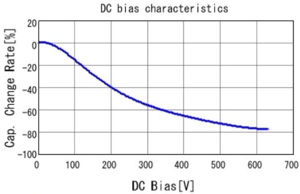
GRM31AR72J222KW01 C-DC bias capchange, 25.0degC, A
