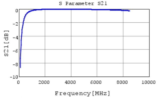
GCQ1555C1H6R3CB01 S21 DCOV, 25degC
