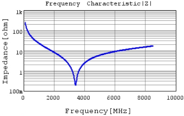
GCQ1555C1H6R3CB01 |Z| DC0V, 25degC
