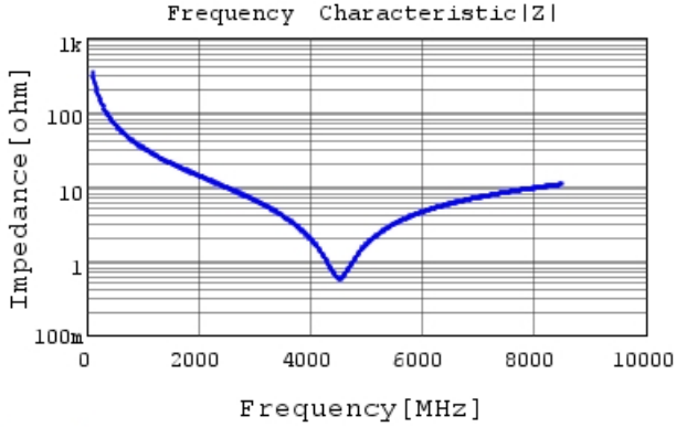
GRM0335C2A4R6BA01 |Z| DCOV, 25degC
