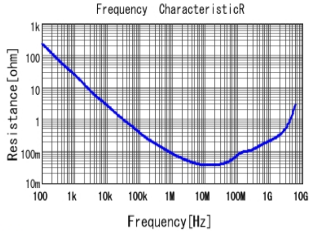
■ GRM155R61A393KA01 R DCOV, 25degC
