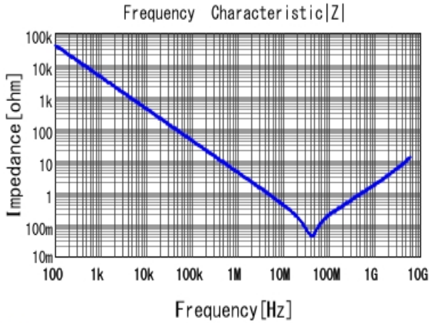
■ GRM155R61A393KA01 |Z| DCOV, 25degC
