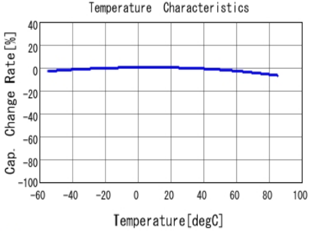
■ GRM155R61A393KA01 C-Temp. capchange, DCO. 0V, AC1.0V rm
