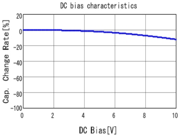
■ GRM155R61A393KA01 C-DC bias capchange, 25.0degC, AC1.
