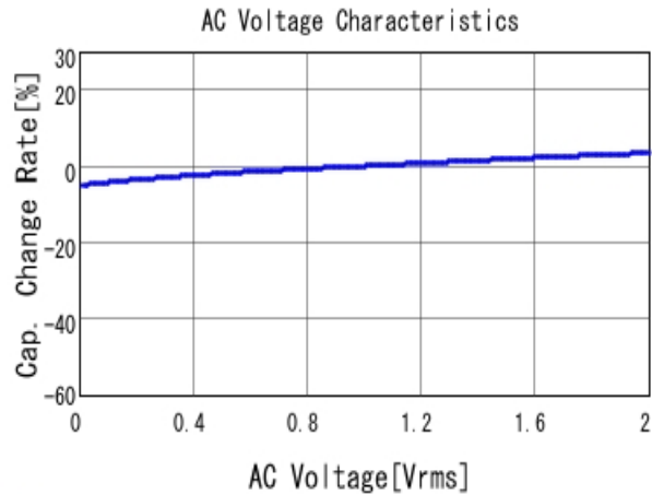
■ GRM155R61A393KA01 C-AC Voltage capchange, DCOV, 25.0d
