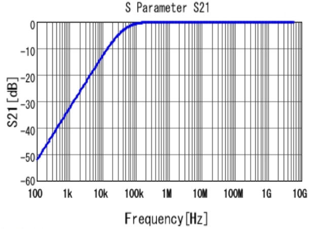
■ GRM155R61A393KA01 S21 DCOV, 25degC
