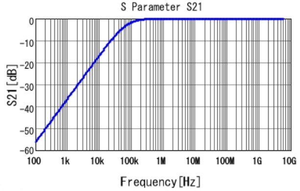
■ GRM033R60J273KE01 S21 DCOV, 25degC
