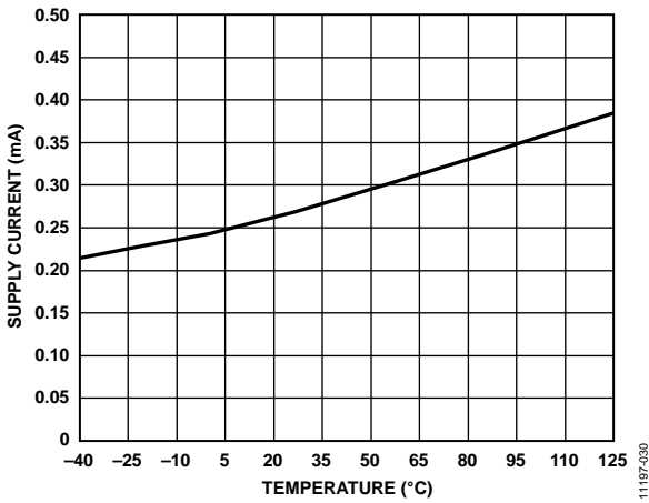
Figure 30. Supply Current vs. Temperature ( G = 1 )
