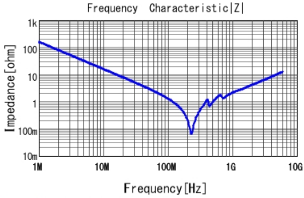
GRM1885C1E102JA01 |Z| DCOV, 25degC
