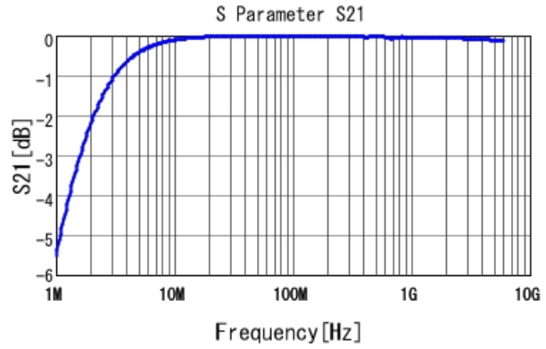
GRM1885C1E102JA01 S21 DCOV, 25degC
