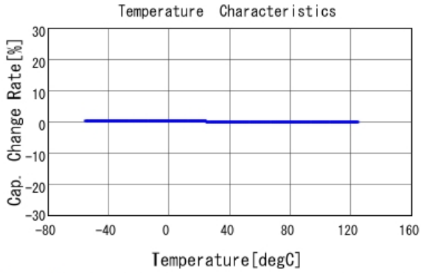
GRM1885C1E102JA01 C-Temp. capchange, DCOV, AC1Vrms
