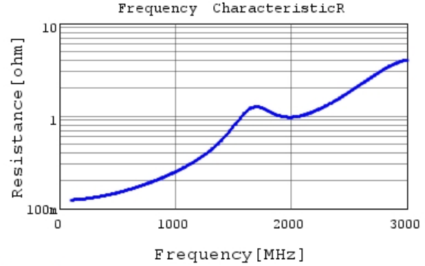
GRM31A7U2J121JW31 R DC0V, 25degC
