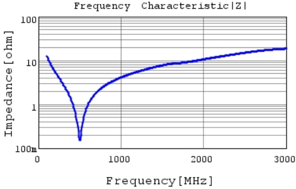
GRM31A7U2J121JW31 |Z| DC0V, 25degC
