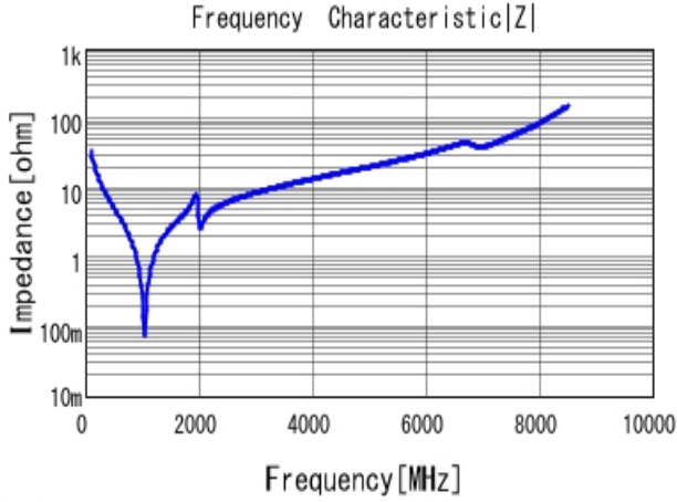
■ GQM1885C1H470JB01 |Z| DC0V, 25degC
