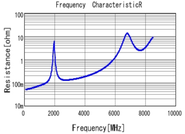
■ GQM1885C1H470JB01 R DC0V, 25degC
