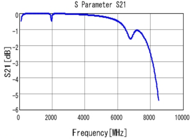
■ GQM1885C1H470JB01 S21 DCOV, 25degC
