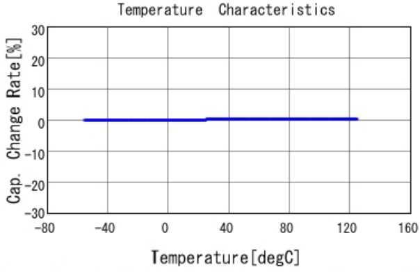
GJM1555C1H1R0WB01 C-Temp. capchange, DCOV, AC1Vrms
