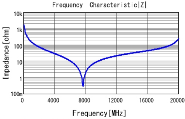
GJM1555C1H1R0WB01 |Z| DCOV, 25degC
