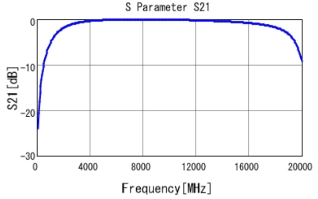
GJM1555C1H1R0WB01 S21 DCOV, 25degC
