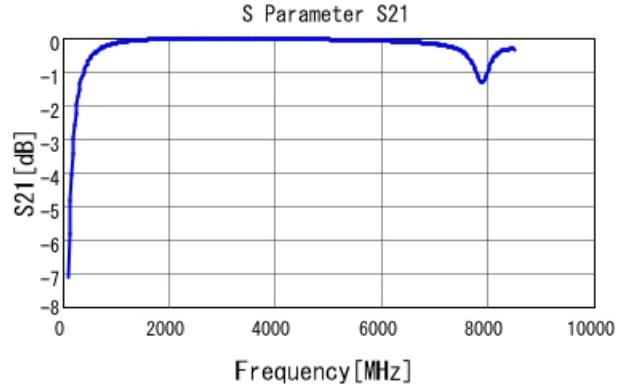
GCQ1555C1H7R8CB01 S21 DC0V, 25degC
