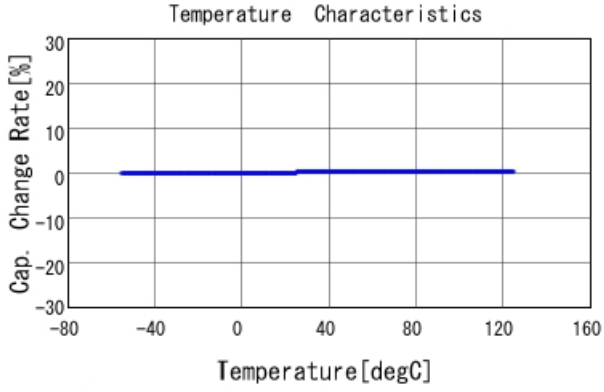
GCQ1555C1H7R8CB01 C-Temp. capchange, DC0V, AC1Vrms
