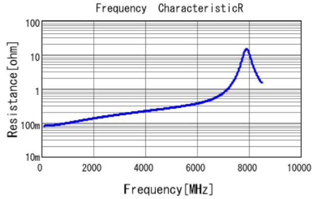
GCQ1555C1H7R8CB01 R DC0V, 25degC
