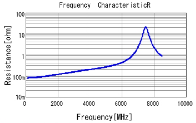
GJM1555C1H8R9BB01 R DCOV, 25degC
