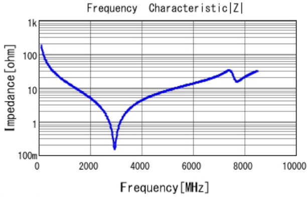
GJM1555C1H8R9BB01 |Z| DCOV, 25degC
