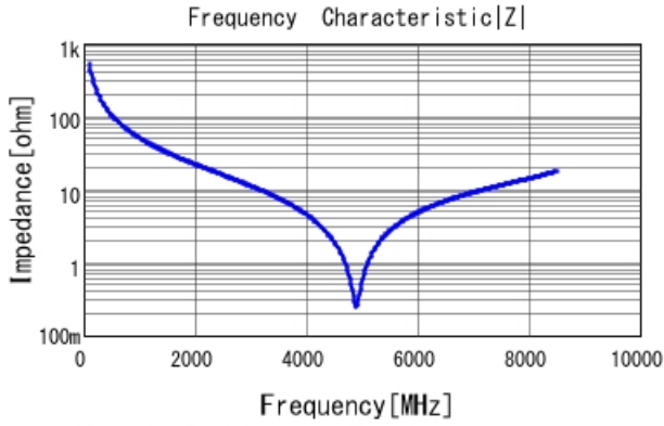
GJM1555C1H3R0WB01 |Z| DCOV, 25degC
