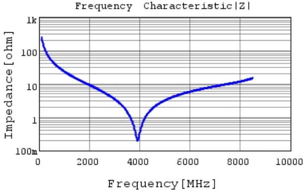
GJM0335C1E6R4DB01 |Z| DC0V, 25degC
