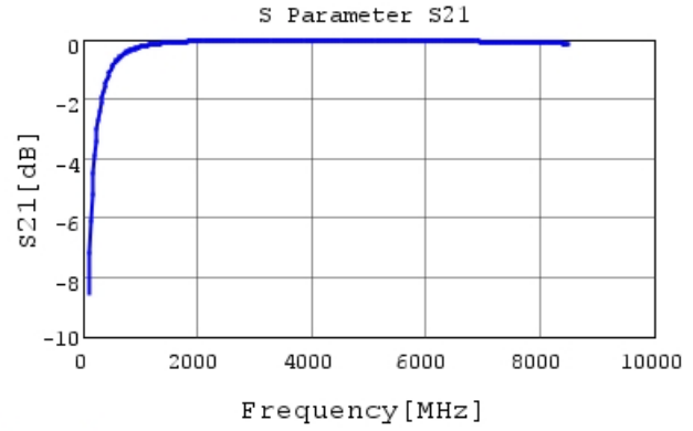
GJM0335C1E6R4DB01 S21 DCOV, 25degC
