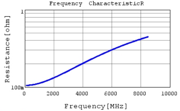
GJM0335C1E6R4DB01 R DC0V, 25degC
