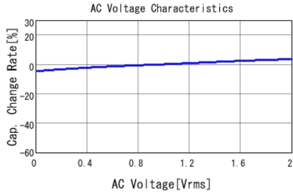
GRM219R71H334KA88 C-AC Voltage capchange, DCOV, 25
