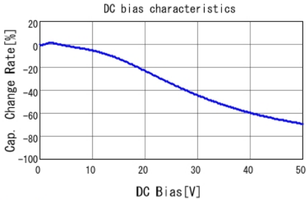
GRM219R71H334KA88 C-DC bias capchange, 25.0degC, A
