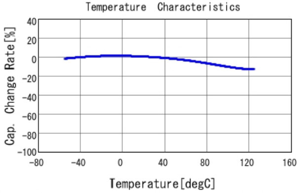
GRM219R71H334KA88 C-Temp. capchange, DC0.0V, AC1.C
