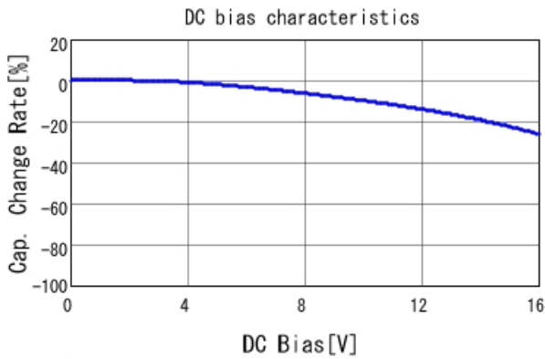
GRT155R71C473KE01 C-DC bias capchange, 25.0degC, A
