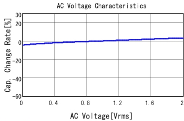
GRT155R71C473KE01 C-AC Voltage capchange, DCOV, 25
