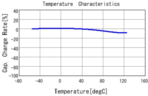
GRT155R71C473KE01 C-Temp. capchange, DC0.0V, AC1.C
