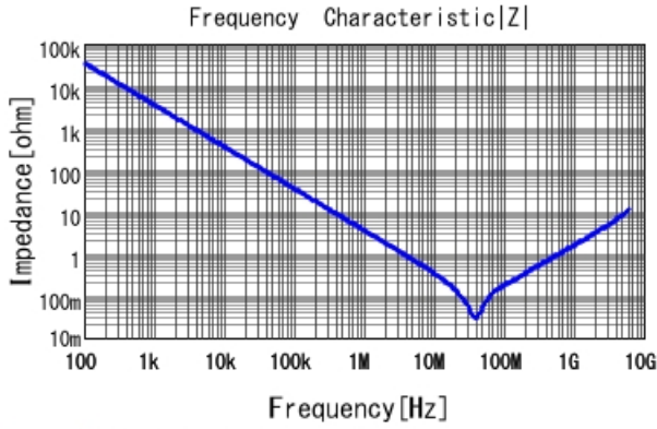
GRT155R71C473KE01 |Z| DCOV, 25degC
