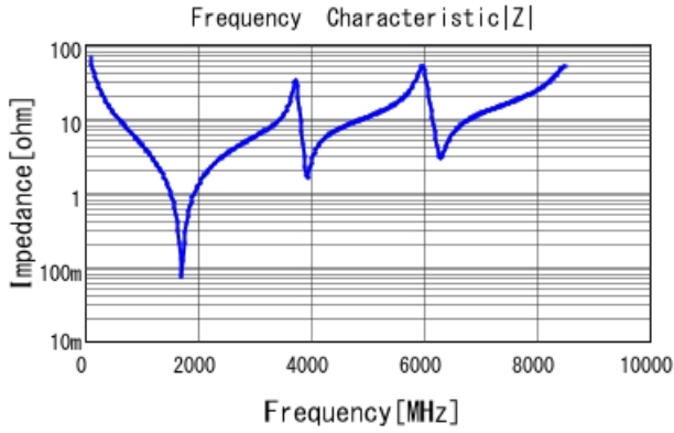
GQM1875C2E240GB12 |Z| DCOV, 25degC
