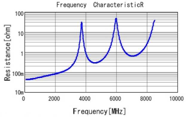
GQM1875C2E240GB12 R DCOV, 25degC
