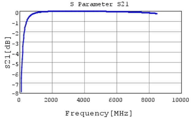
GCQ1555C1H7R0DB01 S21 DCOV, 25degC
