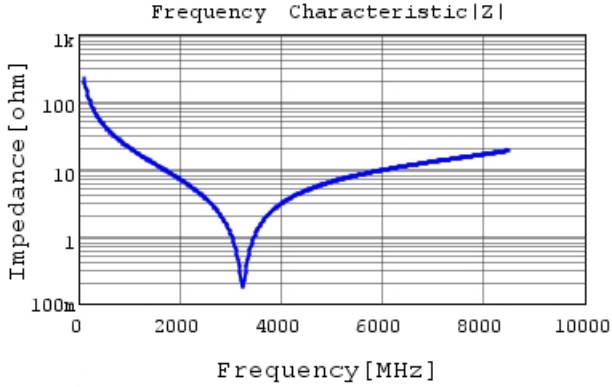
GCQ1555C1H7R0DB01 |Z| DC0V, 25degC
