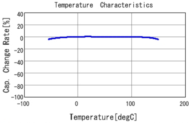
■ GCJ188R92A103MA01 C-Temp. capchange, DCO. 0V, AC1. 0Vrm
