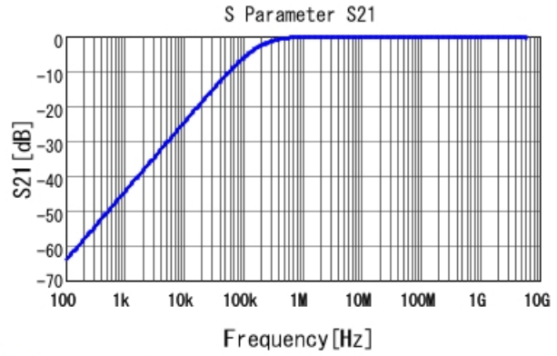
■ GCJ188R92A103MA01 S21 DCOV, 25degC
