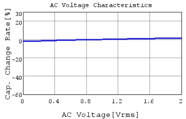
RDER72A152K0M1H03A C-AC Voltage capchange, I
