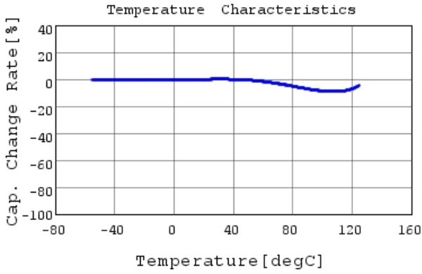
RDER72A152K0M1H03A C-Temp. capchange, DC0.0V
