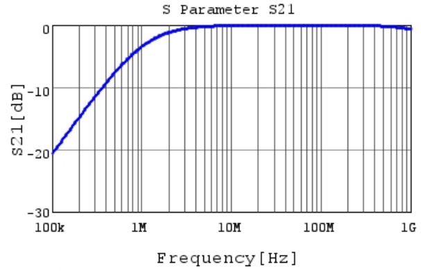
RDER72A152K0M1H03A S21 DC0V, 25degC
