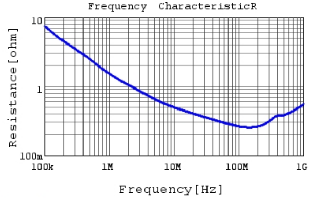
RDER72A152K0M1H03A R DCOV, 25degC
