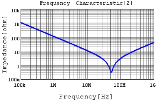
RDER72A152K0M1H03A |Z| DCOV, 25degC
