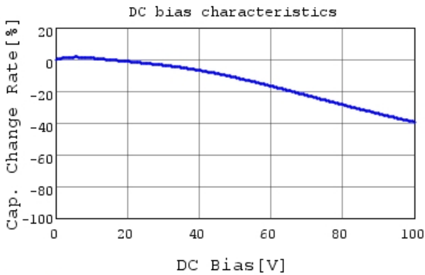
RDER72A152K0M1H03A C-DC bias capchange, 25.0
