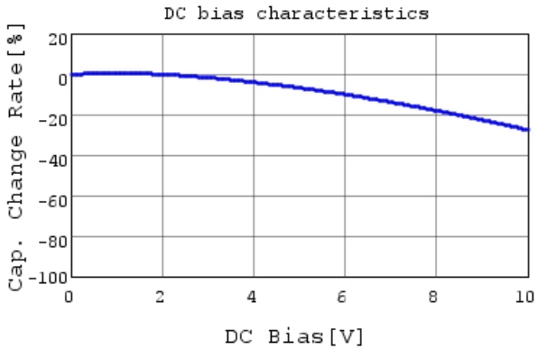
GRM033R61A472MA01 C-DC bias capchange, 25.0c
