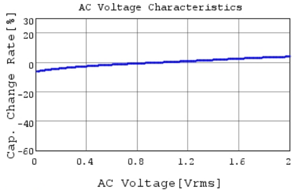
GRM033R61A472MA01 C-AC Voltage capchange, Dc
