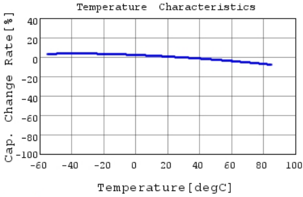
GRM033R61A472MA01 C-Temp. capchange, DC0.0V,
