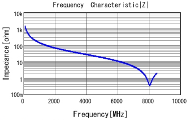
GJM1555C1H1R1BB01 |Z| DCOV, 25degC
