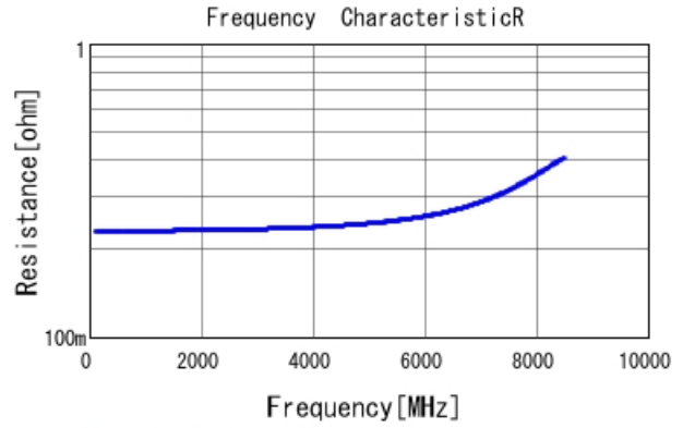
GJM1555C1H1R1BB01 R DCOV, 25degC
