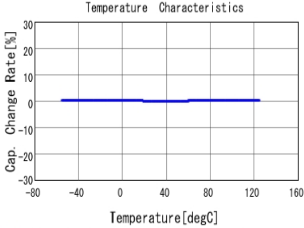
■ GRM1552C1H6R8DA01 C-Temp. capchange, DCOV, AC1Vrms
