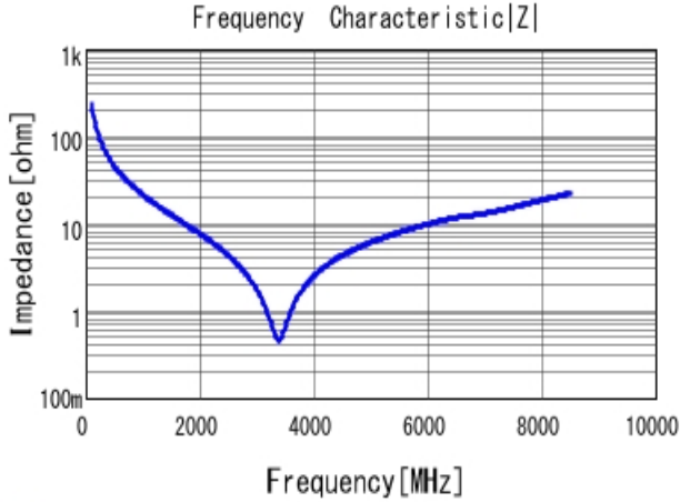
■ GRM1552C1H6R8DA01 |Z| DCOV, 20degC
