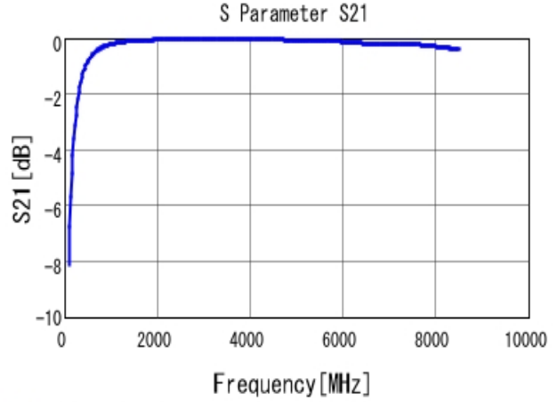
■ GRM1552C1H6R8DA01 S21 DCOV, 20degC
