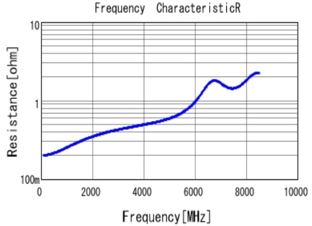
■ GRM1552C1H6R8DA01 R DCOV, 20degC
