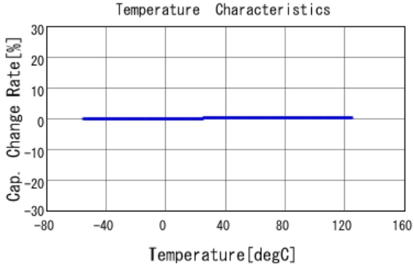
GRM1885C2A9R6BA01 C-Temp. capchange, DCOV, AC1Vrms
