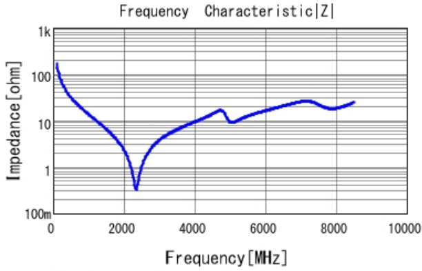
GRM1885C2A9R6BA01 |Z| DCOV, 25degC
