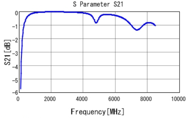
GRM1885C2A9R6BA01 S21 DCOV, 25degC
