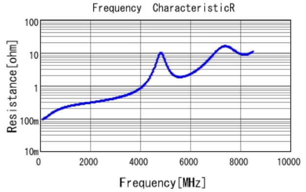
GRM1885C2A9R6BA01 R DCOV, 25degC
