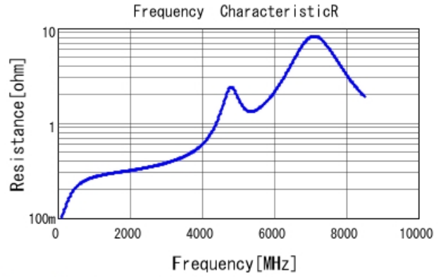
GRM1885C2A9R8CA01 R DCOV, 25degC
