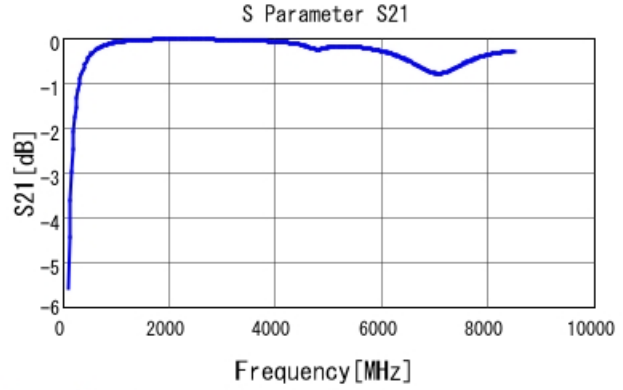
GRM1885C2A9R8CA01 S21 DCOV, 25degC
