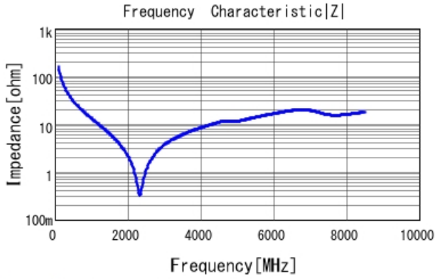
GRM1885C2A9R8CA01 |Z| DCOV, 25degC
