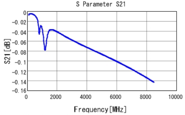
GRM1555C2A471JE01 S21 DCOV, 25degC
