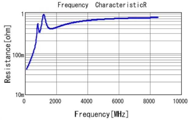
GRM1555C2A471JE01 R DCOV, 25degC
