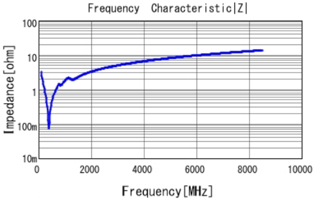
GRM1555C2A471JE01 |Z| DCOV, 25degC
