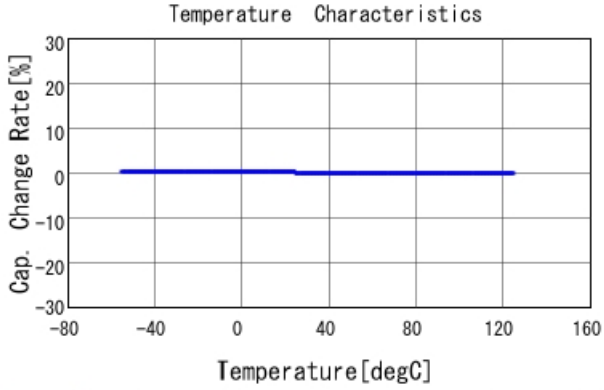
GRM1555C2A471JE01 C-Temp. capchange, DCOV, AC1Vrms
