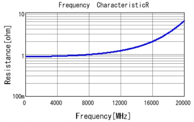
GRM1555C1HR40WA01 R DCOV, 25degC
