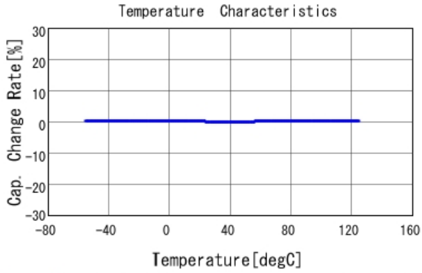
GRM1555C1HR40WA01 C-Temp. capchange, DCOV, AC1Vrms
