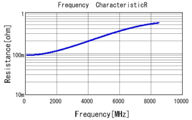
GJM0335C1E5R9WB01 R DCOV, 25degC
