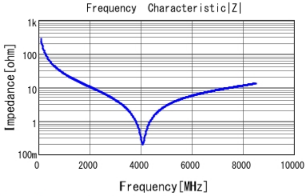
GJM0335C1E5R9WB01 |Z| DCOV, 25degC
