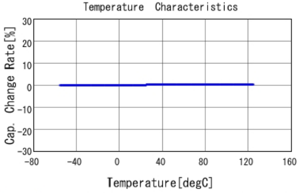
GJM0335C1E5R9WB01 C-Temp. capchange, DC0V, AC1Vrms
