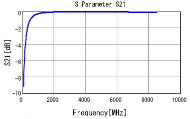
GJM0335C1E5R9WB01 S21 DC0V, 25degC
