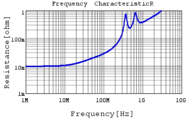
GCM32A7U2J222JX01 R DC0V, 25degC
