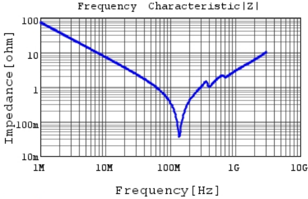
GCM32A7U2J222JX01 |Z| DC0V, 25degC
