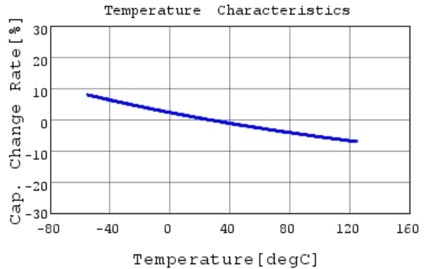
GCM32A7U2J222JX01 C-Temp. capchange, DC0V, 1
