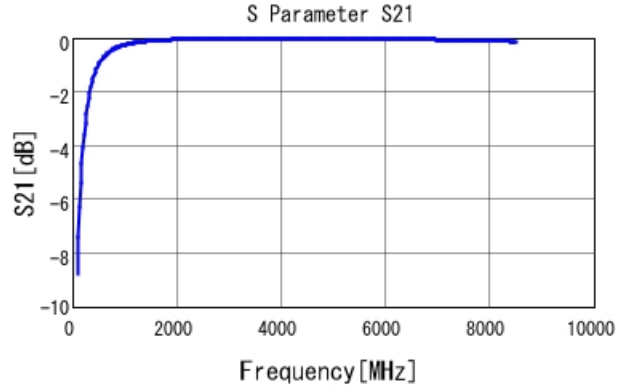
GJM0335C1E6R2BB01 S21 DC0V, 25degC
