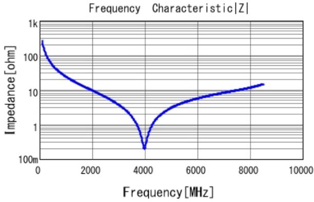
GJM0335C1E6R2BB01 |Z| DCOV, 25degC
