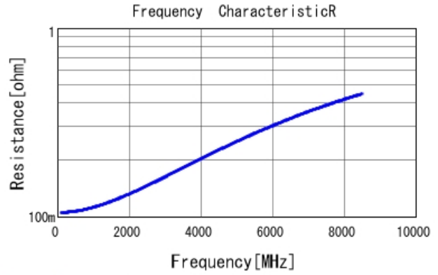
GJM0335C1E6R2BB01 R DCOV, 25degC
