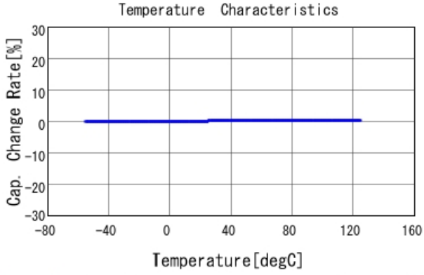
GJM0335C1E6R2BB01 C-Temp. capchange, DC0V, AC1Vrms
