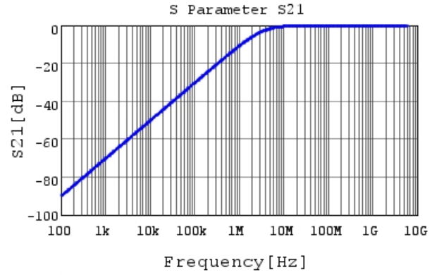
GRM033R71C471KA01 S21 DC0V,25degC
