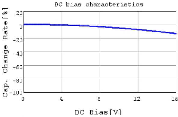
GRM033R71C471KA01 C-DC bias capchange, 25.0c
