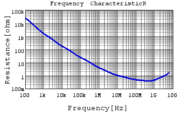
GRM033R71C471KA01 R DCOV, 25degC
