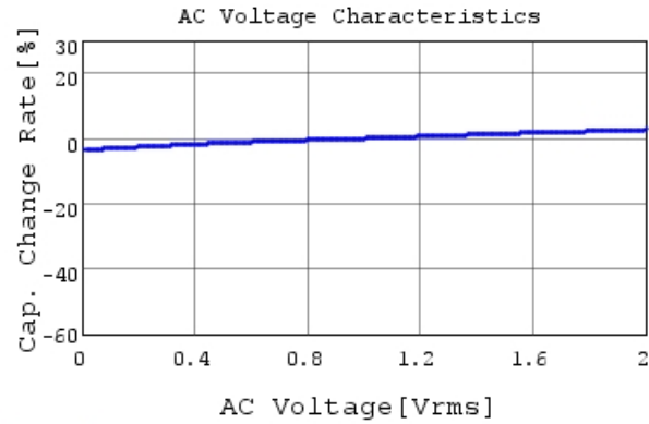
GRM033R71C471KA01 C-AC Voltage capchange, Dc
