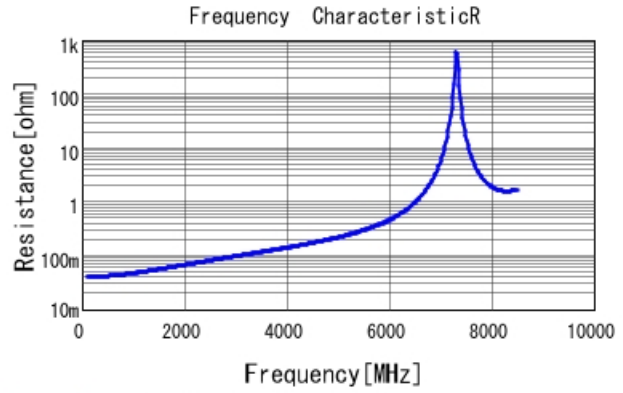
GQM2195C2E4R7CB12 R DCOV, 25degC
