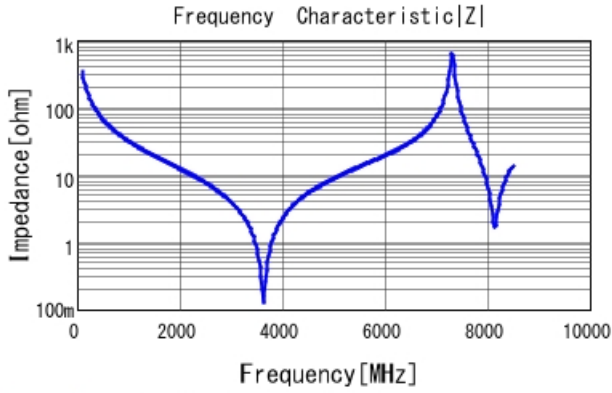
GQM2195C2E4R7CB12 |Z| DCOV, 25degC
