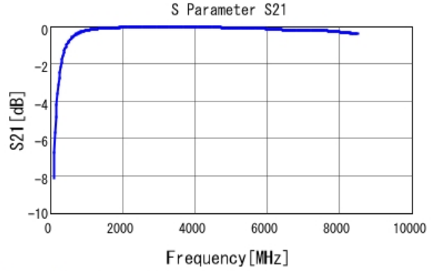
GRM1555C2A6R8DA01 S21 DCOV, 25degC
