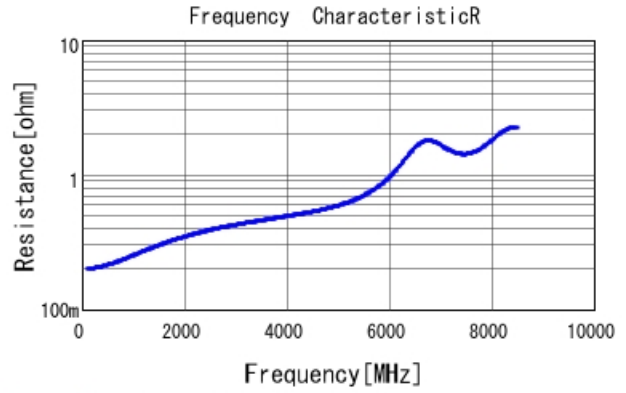
GRM1555C2A6R8DA01 R DCOV, 25degC
