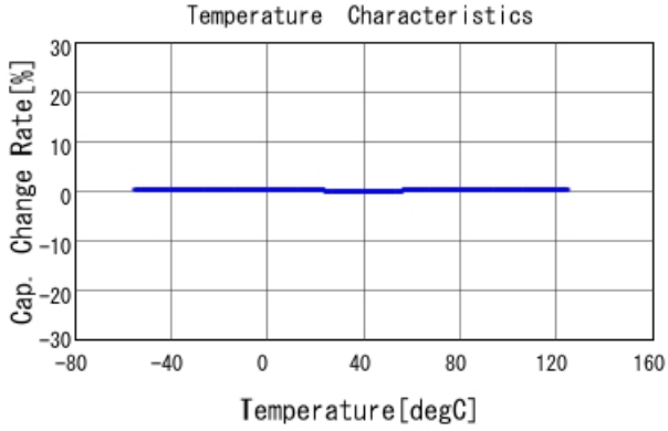
GRM1555C2A6R8DA01 C-Temp. capchange, DCOV, AC1Vrms
