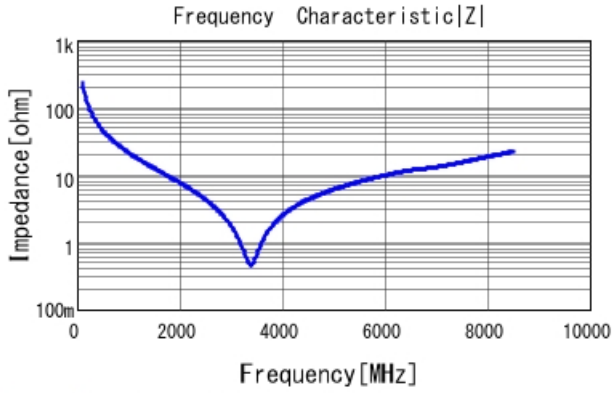
GRM1555C2A6R8DA01 |Z| DCOV, 25degC
