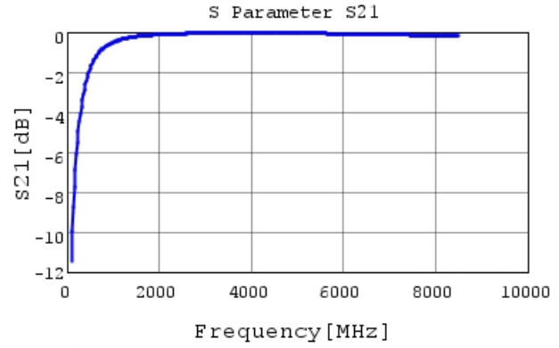
GRM0335C2A4R4BA01 S21 DCOV, 25degC
