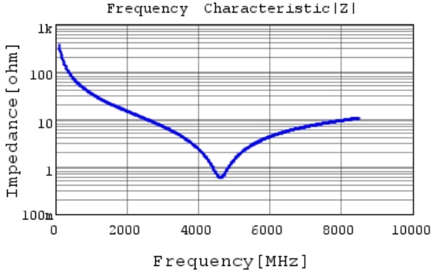
GRM0335C2A4R4BA01 |Z| DC0V, 25degC
