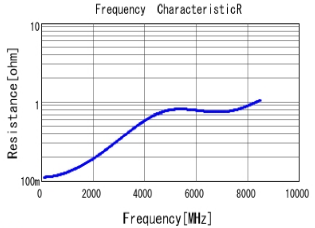
■ GRM0225C1H820JA02 R DC0V, 25degC
