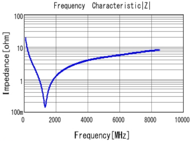
■ GRM0225C1H820JA02 |Z| DC0V, 25degC
