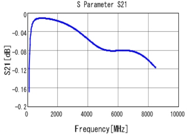
■ GRM0225C1H820JA02 S21 DCOV, 25degC
