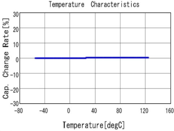
■ GRM0225C1H820JA02 C-Temp. capchange, DCOV, AC1Vrms
